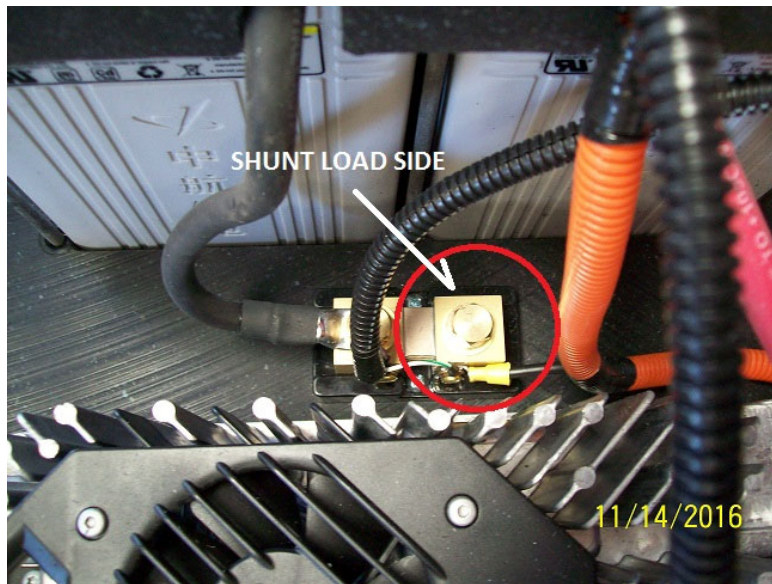
Fig. 23 - Shunt load side
