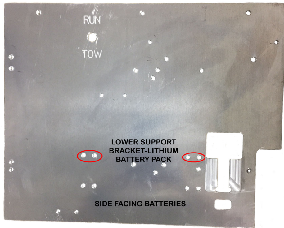
Fig. 12 – Lower Support Bracket Mounting
